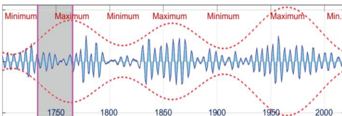
Periods of min. and maximum solar activity from 1700 to 2020 analyzed by machine learning.
